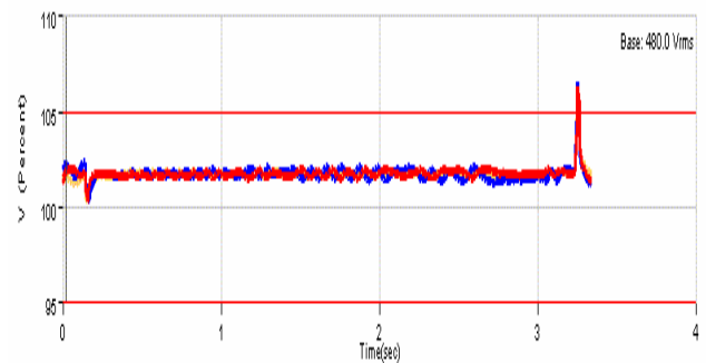
UPS Output
